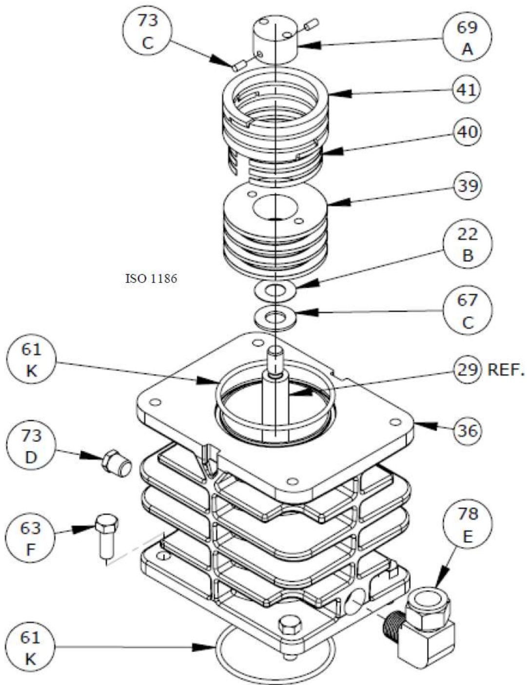
Cylinder Model: NGS082C
