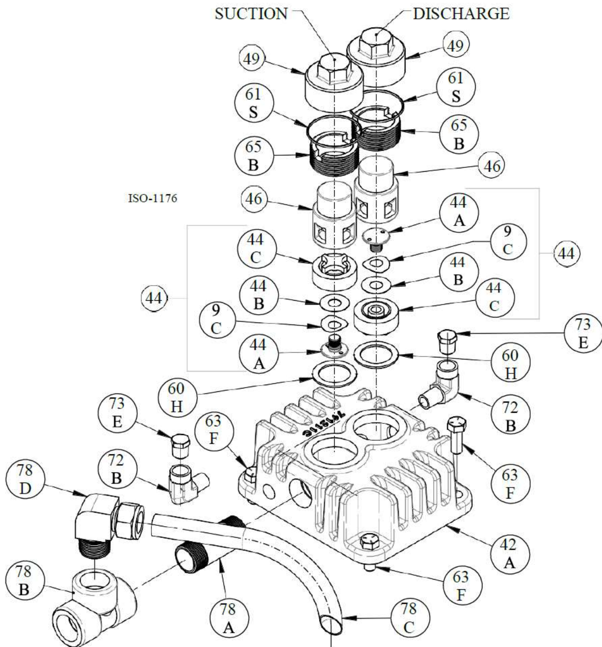
Head Assembly: Model: NGS082
