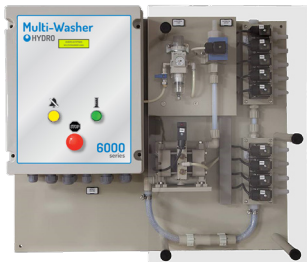
Multi-Washer 6000 Series Pneumatic 1-Channel
