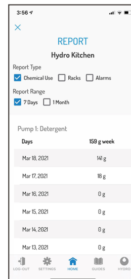
Reports Screen
